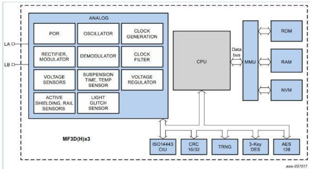
Figure 2. MIFARE DESFire EV3 IC block diagram
